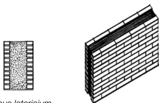
opus latericium
